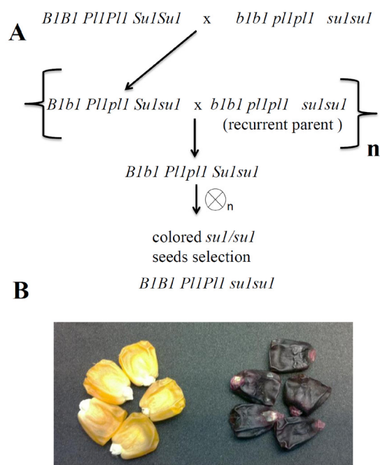
Figure 1 - Breeding scheme. A : Recurrent Selection Scheme: the cross between the B1Pl1 line, source of the regulatory biosynthetic genes and the commercial uncoloured sugary corn gave rise to heterozygous plants for the B-Pl- genes. Among them, the highest anthocyanin content plants were selected for the backcrossing with the recurrent parent. Then the best plants underwent some cycles of self-pollination. B : Phenotype of uncoloured (left) and coloured (right) sweet corn kernels.
