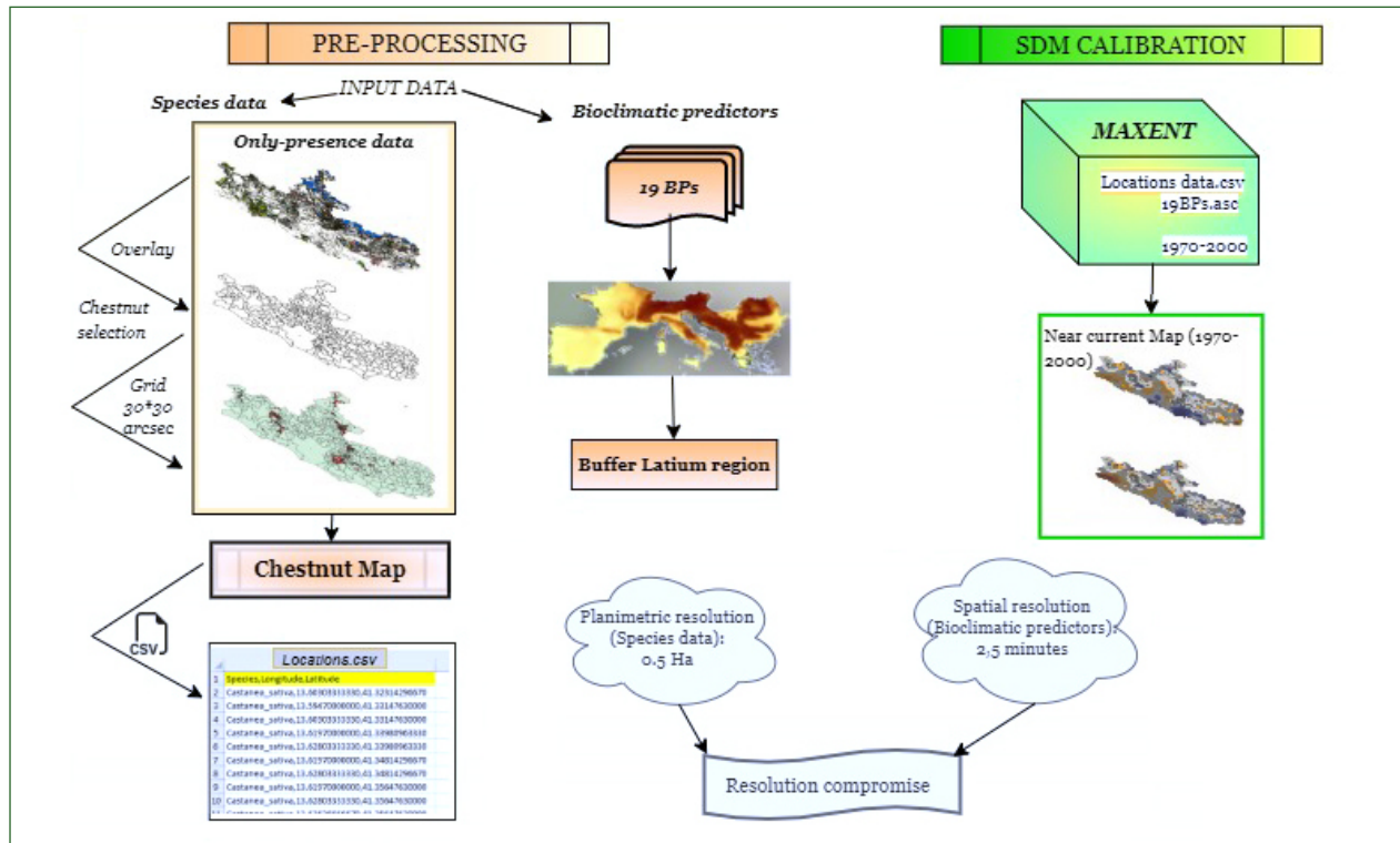
Figure 1 - Pre-processing flowchart.
