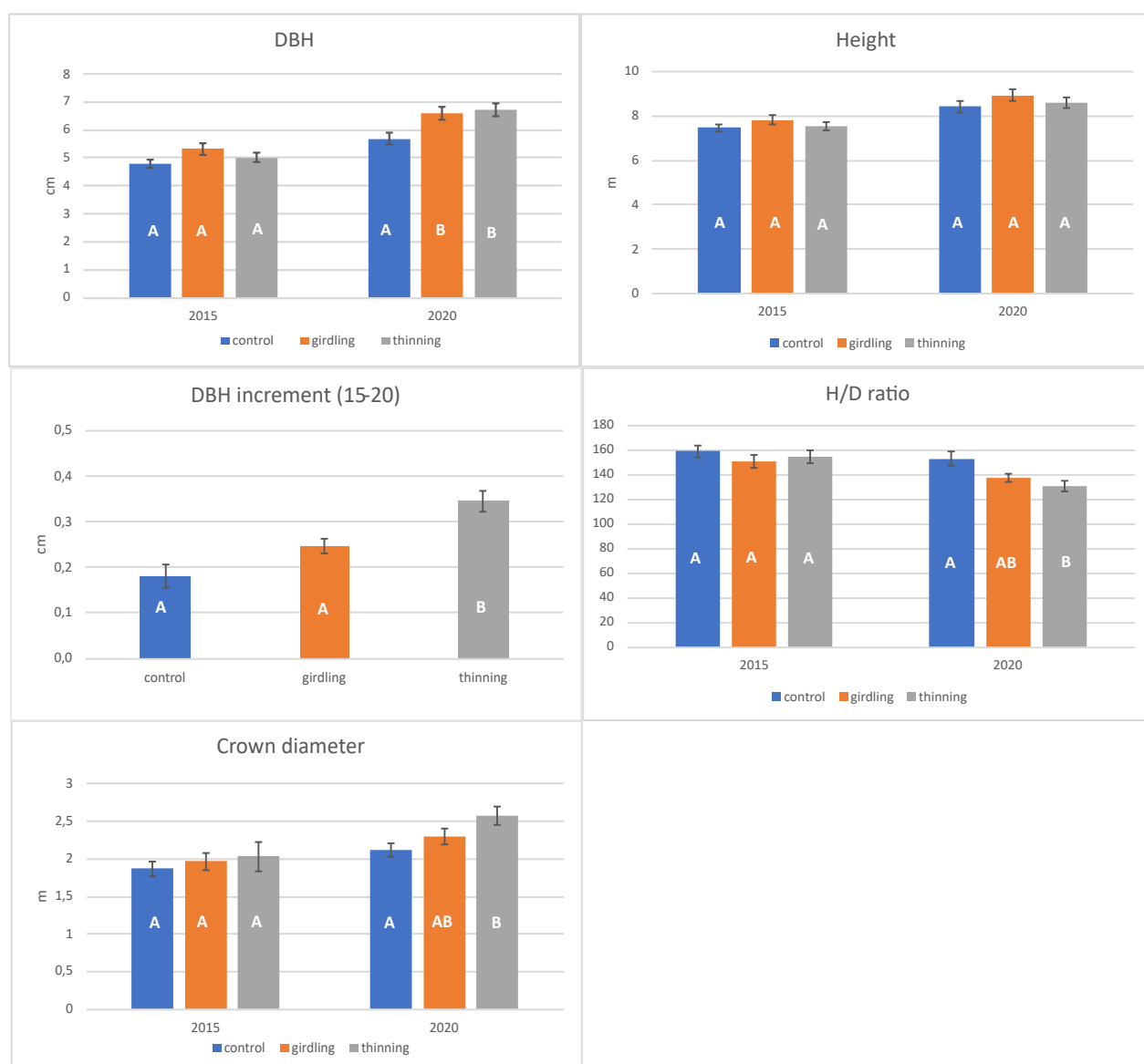
Figure 6 - Mean dasometric parameters \pm st. err. of the selected service trees in the two inventories with the result of the HSD Turkey test.
