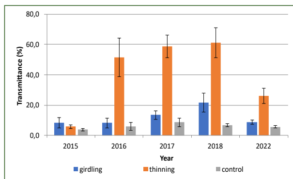
Figure 7 - Transmittance trend per silvicultural treatment under the canopy of the selected sporadic trees before the application of the treatments in 2015 and after the application in the following three years between 2016-2018 and in 2022.
