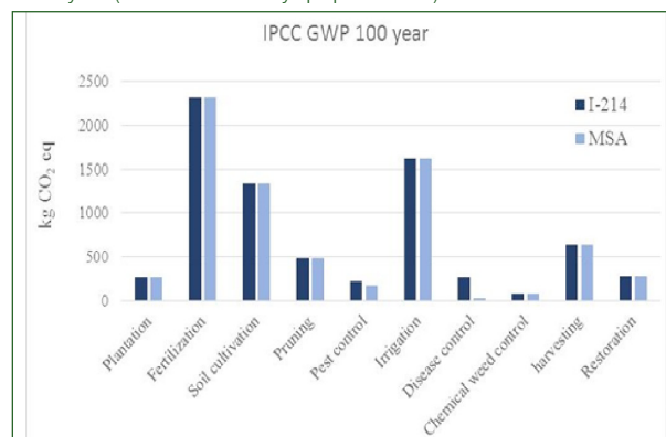
Figure 4 - CO 2 equivalent emissions for 'I-214' and MSA cultivation divided by cultural inputs. Total emissions of the whole cultivation cycle (stooled+nursery+poplar stand).
