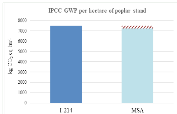
Figure 3 - CO 2 equivalent emissions for 'I-214' and MSA cultivation. Total emissions of the whole cultivation cycle (stooled+nursery+poplar stand). In red striped the emission avoided choosing the cultivation of MSA.
