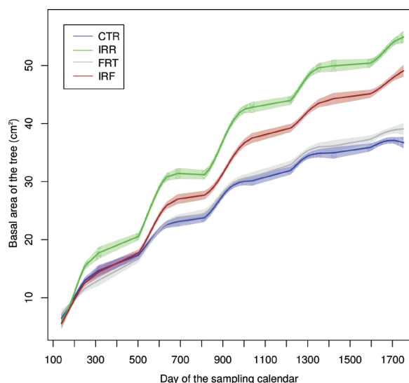
Figure 2 - Growth of diameters at breast height (Dbh) of the trees of each treatment during the five years of measurements. X axis: days of growth (Giulian calendar); y axis: mean basal area (cm²/trees). Shaded area: estimated standard error.
